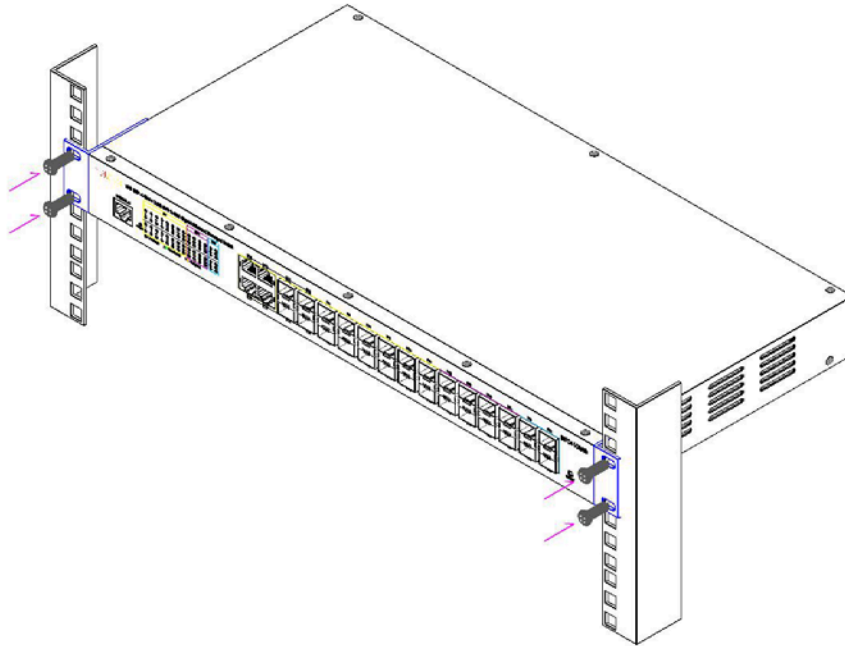
SFC4100A Series Rack Mounting Diagram
